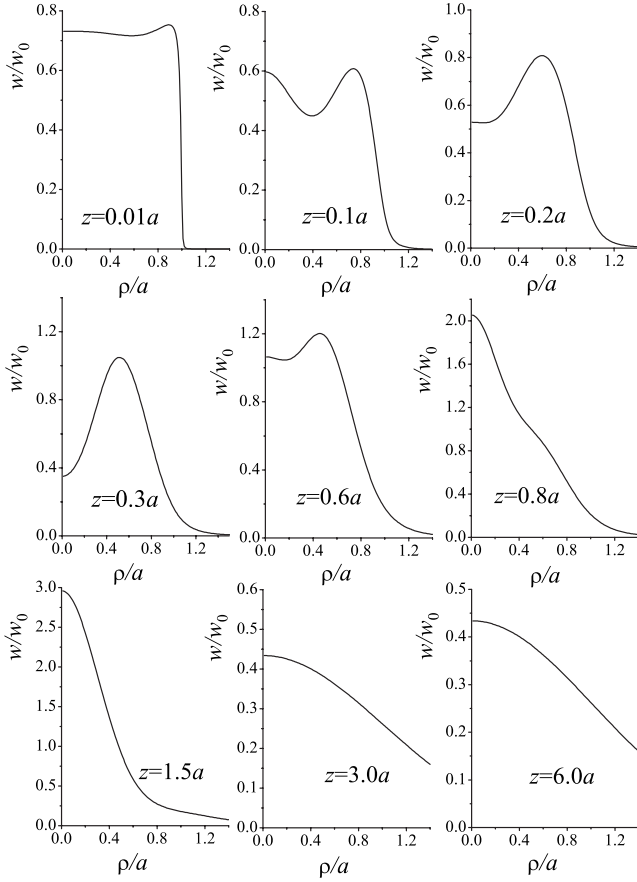
FIG. 7. Transverse profiles of the electric energy density for the Fresnel-atom microlens at ka=8 and different values of longitudinal coordinate z .
