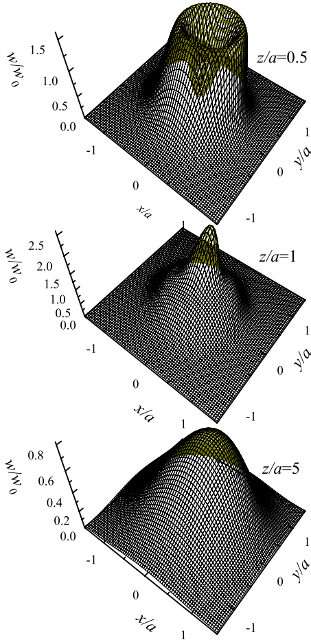
FIG. 5. (Color online) Electric energy density for the Fresnel-atom microlens at ka=10 and at distances from the screen z=0.5a , z=1a , and z=5a .
