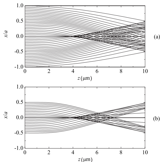
FIG. 11. (a) Atom trajectories in an atomic beam focused by the Fresnel-atom microlens with relative aperture ka=10 at detuning \delta=-300\gamma , laser light intensity I=25 W/cm 2 , and longitudinal atomic beam velocity V=5 m/s. (b) Atom trajectories when the outer part of the atomic beam is blocked by the screen with aperture of radius r<0.5a for the same parameters as in (a).
