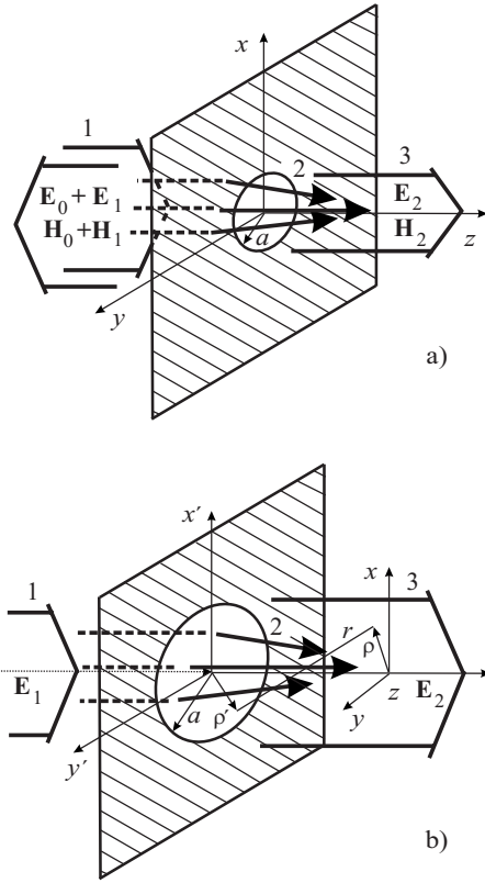
FIG. 1. (a) Bethe-type atom microlens. 1: the field produced by the incident laser light and the light reflected from the aperture, 2: focused atomic beam, 3: the field of the light transmitted through the aperture. (b) Fresnel-type atom microlens. 1: the incident laser light, 2: focused atomic beam, 3: the field of the light transmitted through the aperture.
