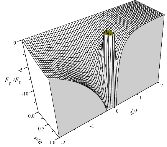
FIG. 8. (Color online) Radial component of the gradient force in case of the Bethe-atom microlens as a function of coordinates at ka=0.25 and for circular polarized incident laser wave.
