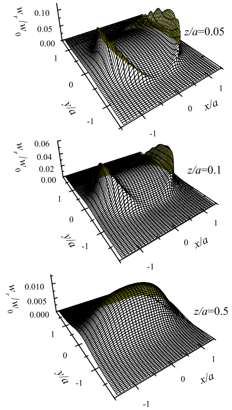
FIG. 2. (Color online) Electric energy density as a function of transverse coordinates in the case of incidence of a linearly polarized light wave on a screen with a circular aperture at ka=0.25 and at distances from the aperture z=0.05a , 0.1a , and 0.5a .
