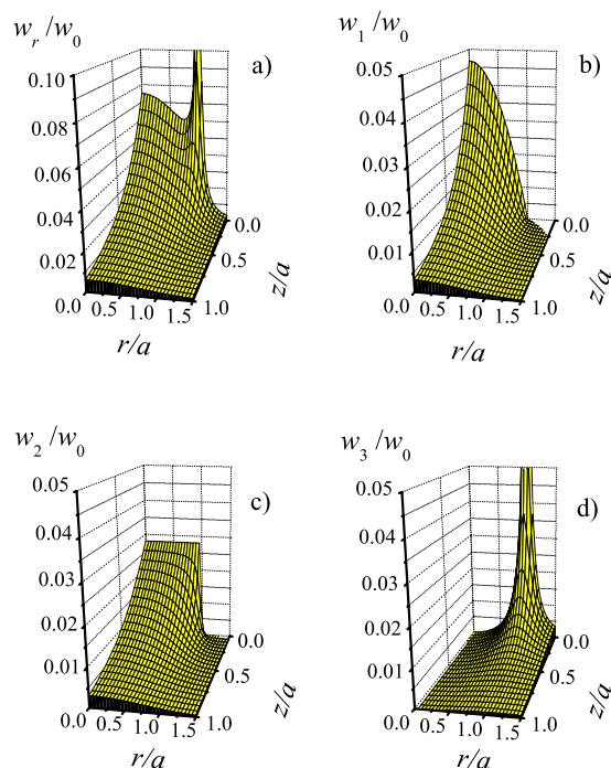
FIG. 4. (Color online) Electric energy density on the right of the screen in case of a circular polarized incident light wave at ka = 0.25 (a) and contributions to the electric energy density of the first (b), second (c), and third (d) term of Eq. (39).
