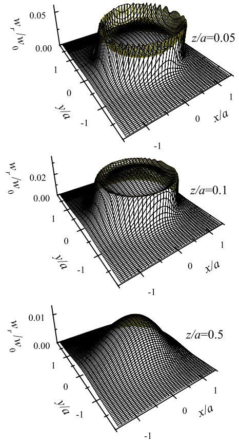
FIG. 3. (Color online) Electric energy density as a function of transverse coordinates in the case of incidence of a circularly polarized light wave on a screen with a circular aperture at ka=0.25 and at distances from the aperture z=0.05a , 0.1a , and 0.5a .
