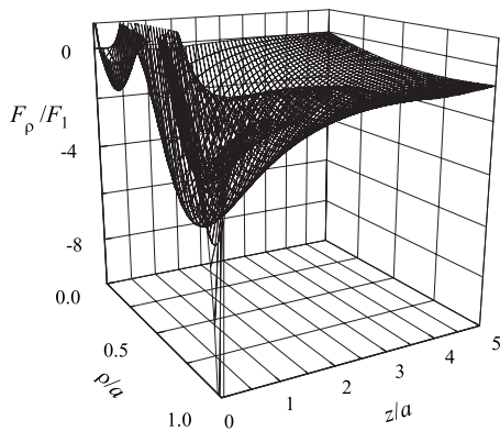
FIG. 9. Radial component of the gradient force in case of the Fresnel-atom microlens as a function of coordinates at ka=10 .
