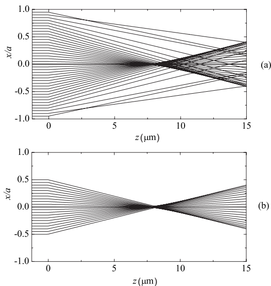
FIG. 10. (a) Atom trajectories in the atomic beam focused by the Bethe-atom microlens. The screen with a round aperture of a relative size ka=0.25 is illuminated by a circularly polarized light wave at detuning \delta=-300\gamma and intensity I=25 W/cm 2 . The longitudinal velocity of atoms is V=5 m/s. (b) Atom trajectories in the same Bethe-atom microlens in the case of blocking of the periphery atoms by an additional screen with a round aperture of radius r=0.5a .
