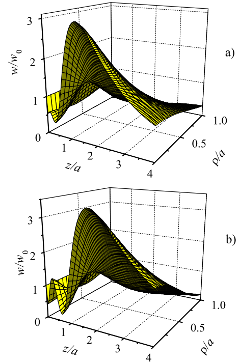
FIG. 6. (Color online) Electric energy density for the Fresnel-atom lens at ka=8 (a) and ka=11 (b).
